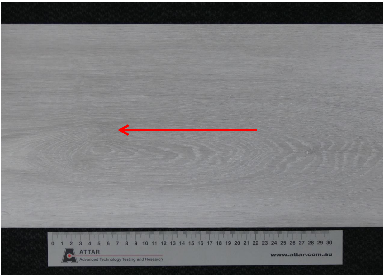
Figure 1: Elemental Dryback - XL, Chevron Herringbone, Loose Lay Arrow indicates direction of testing
