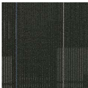
Shaw Diffuse Magnetic Fields
