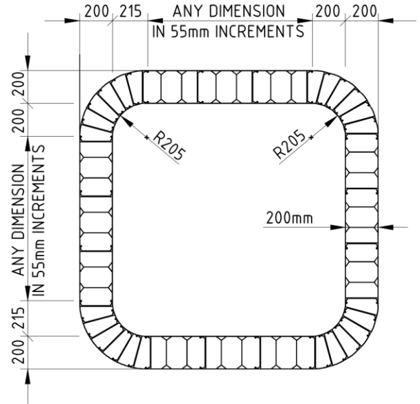
RECTANGULAR OR SQUARE TANK
