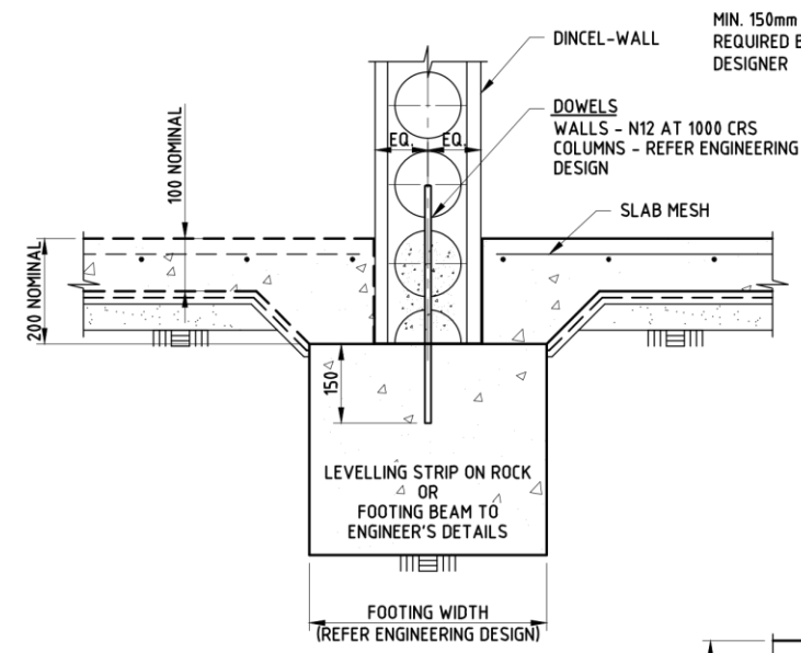
INTERNAL FOOTING DETAIL
