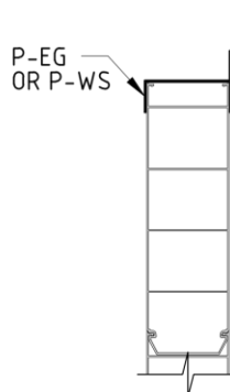
110mm OR 155mm SILL DETAIL
