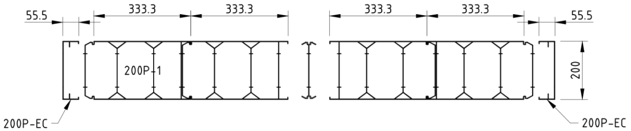
PLAN - WALL ASSEMBLY - WATERPROOF WALL RECOMMENDED FOR BUILDING BASEMENT/FACADE WALLS
