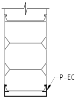
200mm HEAD DETAIL
