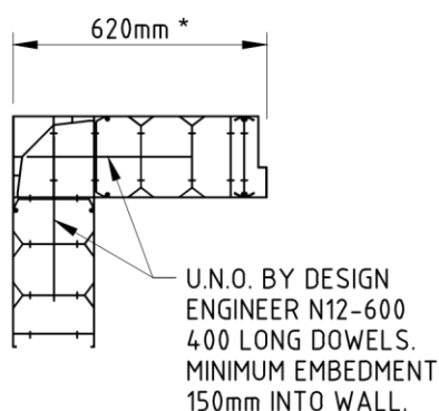
PLAN- CORNERS
