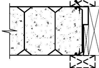
WINDOW JAMB-PLAN
