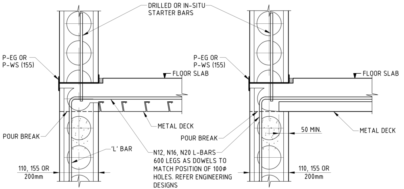
ALTERNATIVE DETAIL -2 EXTERNAL WALL
