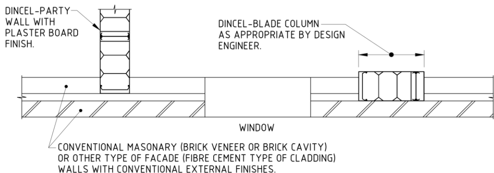
FACADE WALL - OPTION 3
