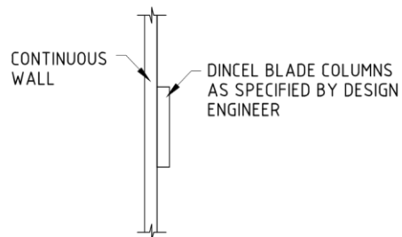
PLAN AT OPTION 1
