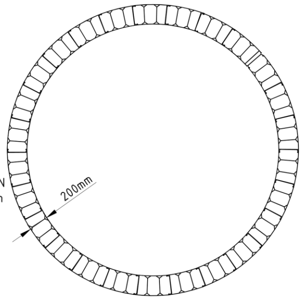
CIRCULAR TANK
