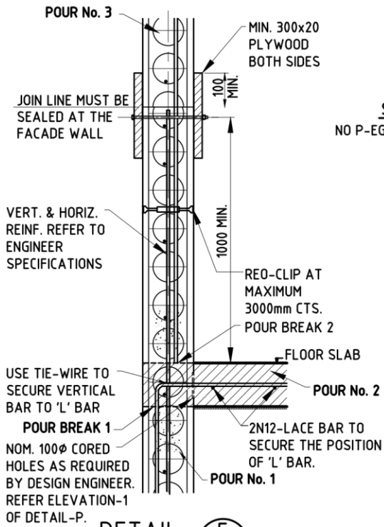
DETAIL 5
