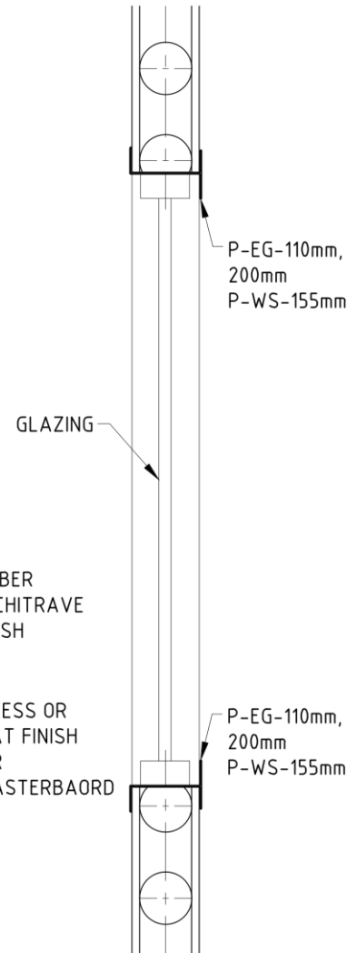
DETAIL AT HEAD & SILL
