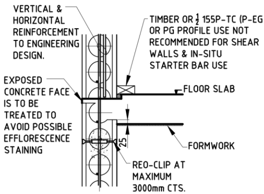
DETAIL 4
