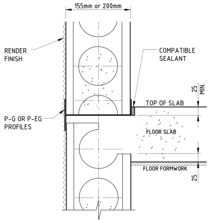
OPTIONAL DETAIL AT FACADE WALL OR SLAB EDGE
