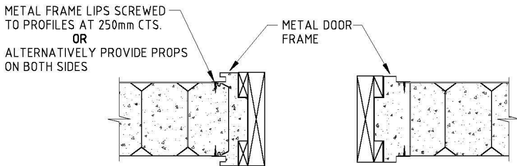
PLAN AT METAL DOOR FRAMES
