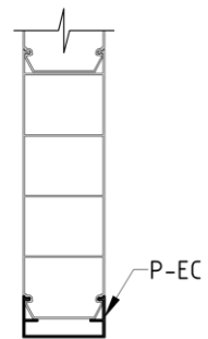
110mm OR 155mm HEAD DETAIL
