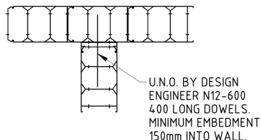
PLAN- 'T' JUNCTIONS
