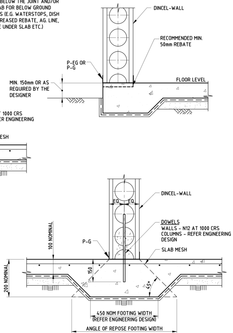
INTERNAL FOOTING DETAIL
