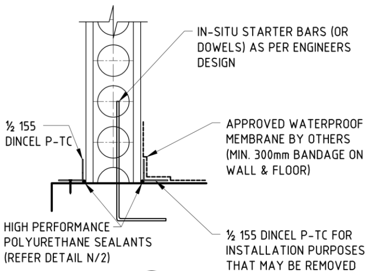
DETAIL 1
