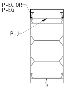
200mm SILL DETAIL
