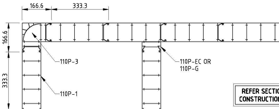
110mm CORNER ASSEMBLY
