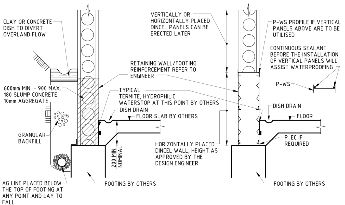
CONVENTIONAL VERTICALLY PLACED DINCEL BASEMENT WALL
