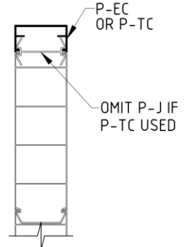
110mm OR 155mm SILL DETAIL
