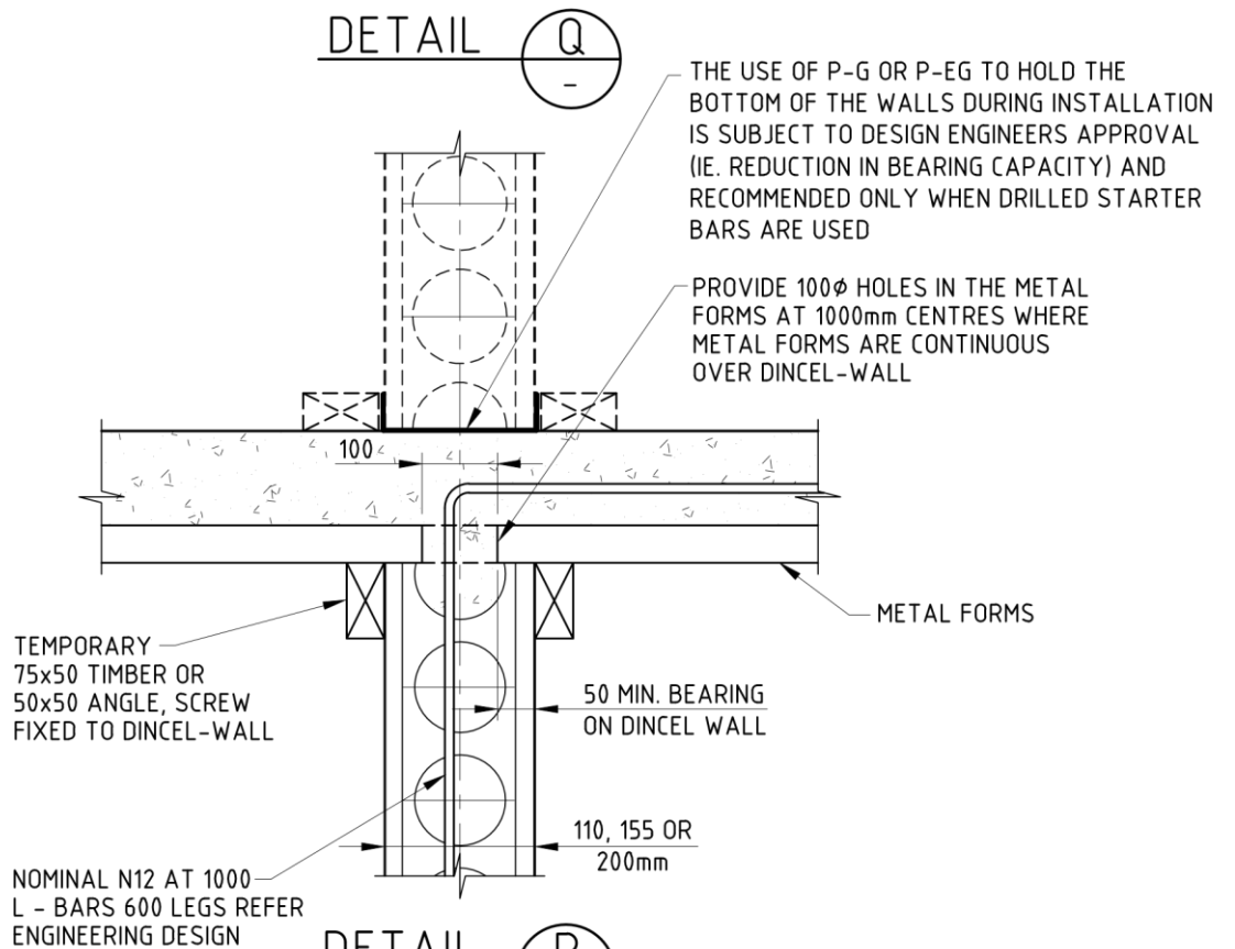
DETAIL R
