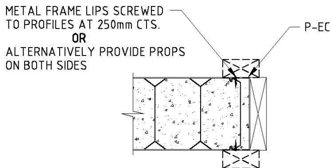
PLAN- SQUARE FINISH WITHOUT DOOR FRAME
