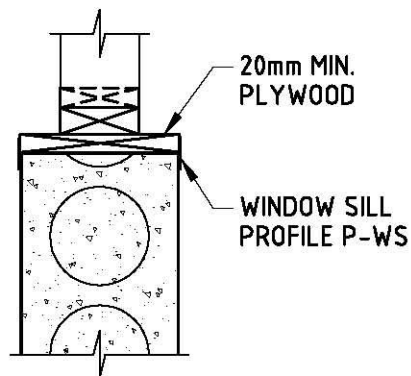
SILL SECTION
