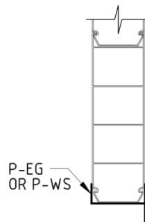
110mm OR 155mm HEAD DETAIL
