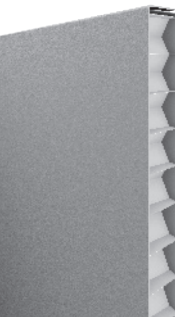
QC50 Two folded aluminium layers with honeycomb core inside
