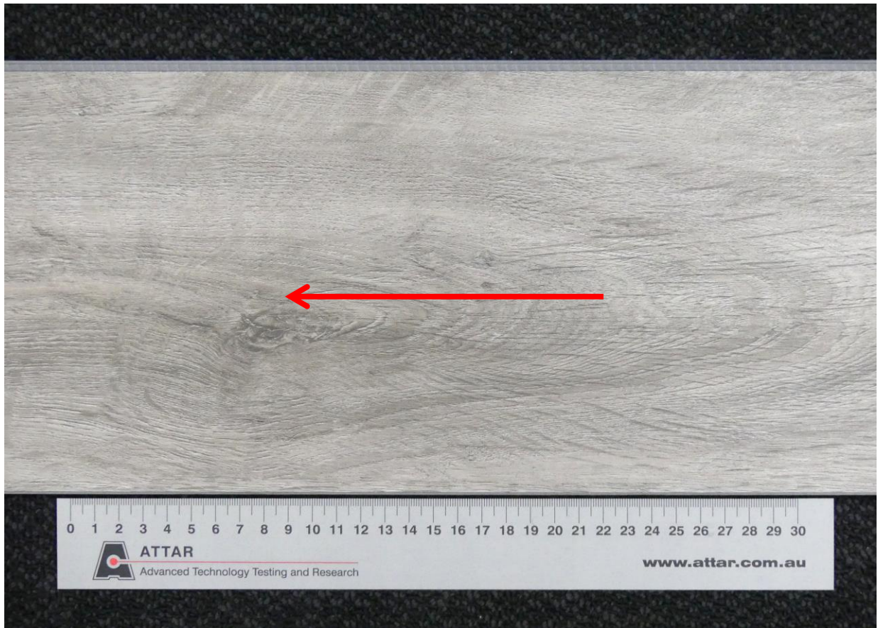
Figure 1: Emboss Code DG - GD - F12 vinyl plank Arrow indicates direction of testing
