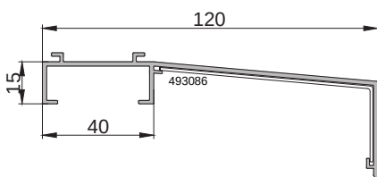
499080 adapter profile with 80mm window sill
