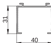
494031 adapter profile for window sill
