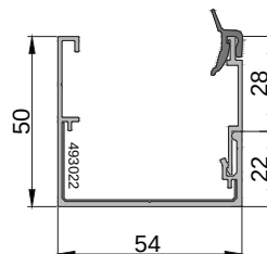
420040 top and lateral frame profile
